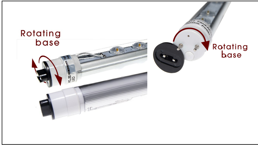
Application: Designed specifically for sign industry, 2 side/face commercial signs. Rotating HO base.
